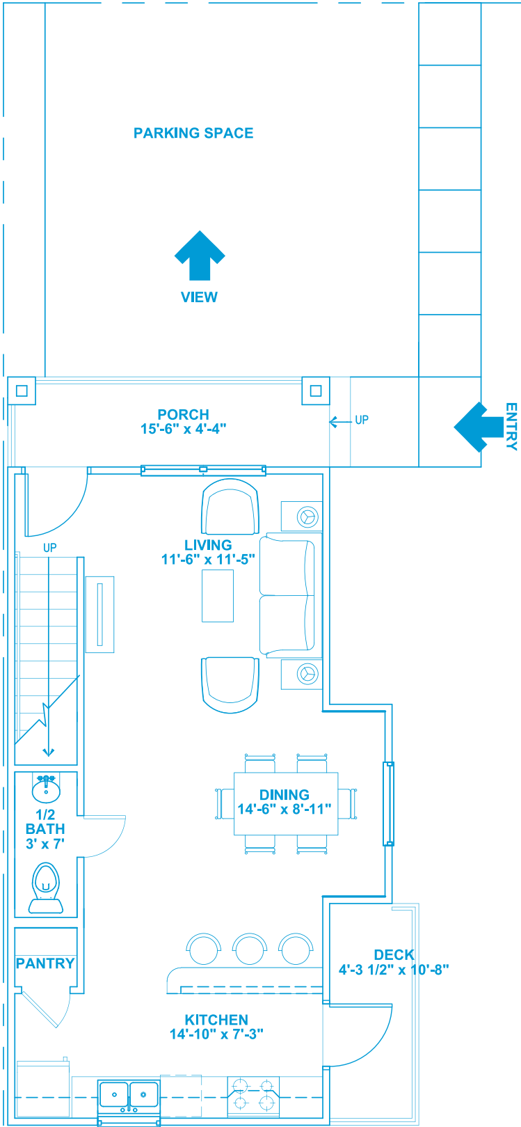
1 ST FLOOR
