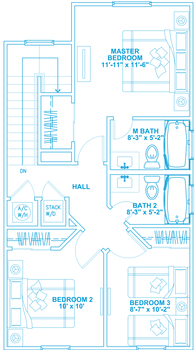
2 ND FLOOR
