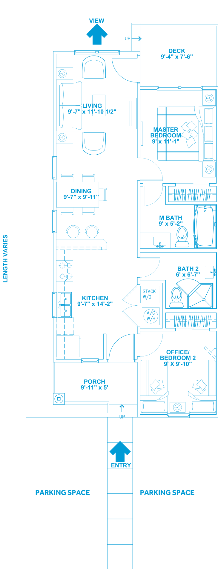
1 ST FLOOR
