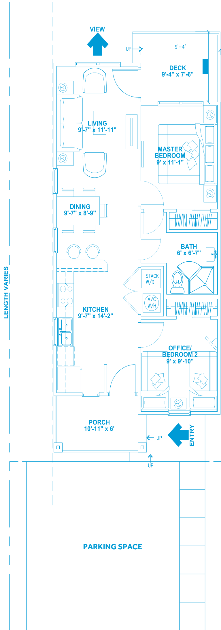
1 ST FLOOR
